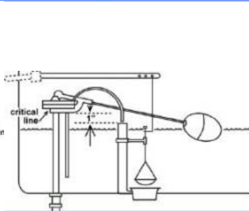
Anti-Siphon Ball-Cock
